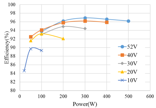
Fig. 16. Efficiency curves with different output voltages.
